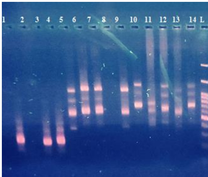
Fig 3. Electrophoresis gel of studied ecotypes from DNA fragments produced by SCoT-18 https://doi.org/10.2298/GENSR2103391E
