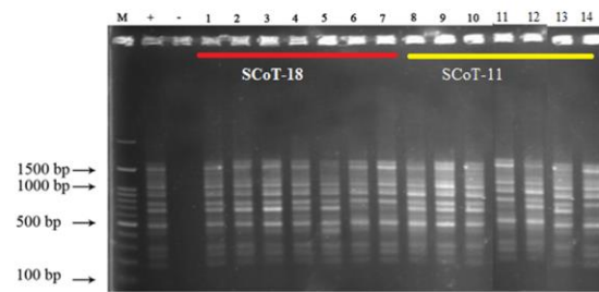
Fig 3. Electrophoresis gel of studied ecotypes from DNA fragments produced by SCoT-18 https://doi.org/10.2298/GENSR2102895L
